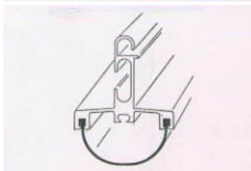
EXTRUDED ALUMINUM BOTTOM BAR ASSMYS. WITH VINYL ASTRAGAL
